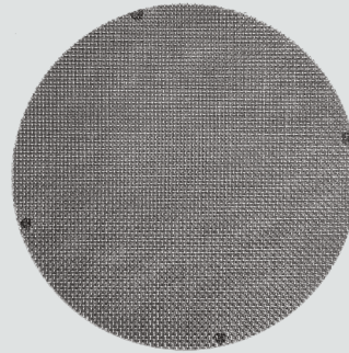
Weld-packs – for increased bend resistance and pack integrity.
