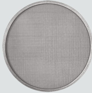
Bound screens – seamless frame of soft aluminum for a better seal at the edge of the breaker plate.
